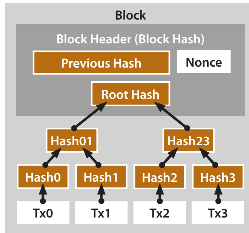
Transactions Hashed in a Merkle Tree
